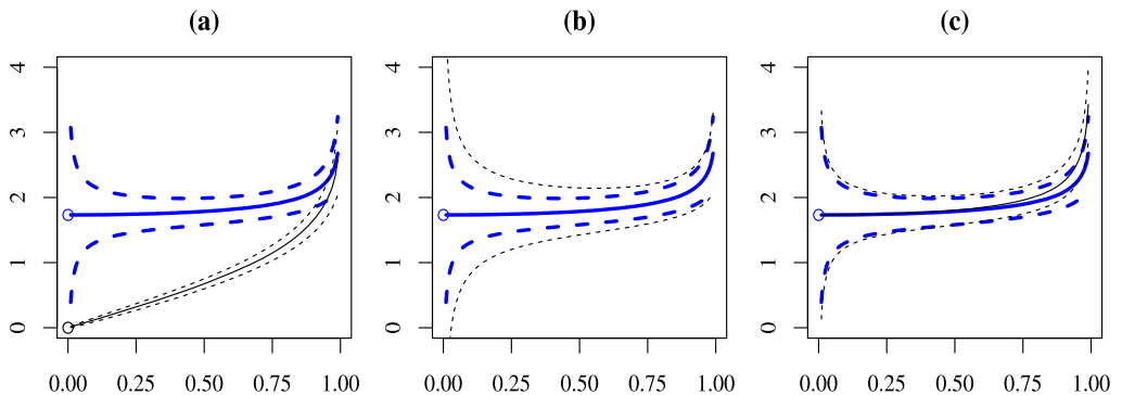
Figure 1. Compares the asymptotic distribution of \hat{z}_\psi/\hat{\sigma}_\psi for a normal reference distribution (thick line) with (a) \hat{z}_\psi/\hat{\sigma}_{\psi, \text{corr}} using the corrected scale estimator, (b) \hat{z}_\psi/(\sigma \varsigma_\psi) using the known scale, and (c) \hat{z}_\psi/\hat{\sigma}_\psi for a t(5) reference distribution. The solid lines indicate the mean, the dashed lines indicate the 5% and 95% asymptotic quantiles for n = 128 .
